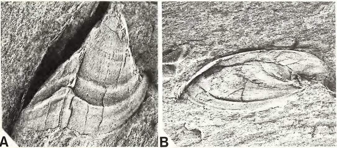
TEXT-FIG. 2. Telamocornu cambriense (Belt, 1868). Upper Ffestiniog Flags Formation; \times 3 ; BM62087. A, lectotype; fragment of dorsal surface showing transverse rugae and median sinus. B, paralectotype; lateral view of specimen crushed in shale.
